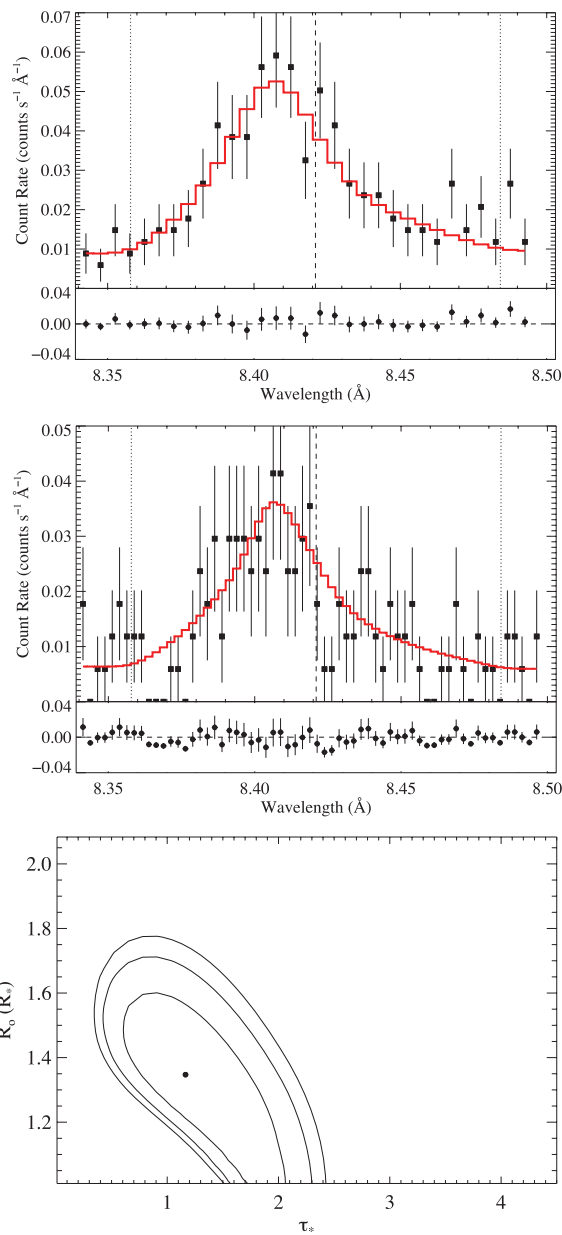
Figure 7. The derived value of \tau_* is also low for the Mg XII Ly \alpha line at 8.421 Å shown here, but it is modestly higher than the shorter wavelength Si XIII complex shown in the previous figure.
