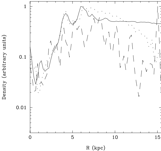
FIG. 3.—Profiles of gas density as a function of galactocentric radius that are used to generate the models described in the text. Profiles are shown for 1.2 \text{ kpc} < z < 2.1 \text{ kpc} (solid line), 2.1 \text{ kpc} < z < 3.0 \text{ kpc} (dashed line), and 3.0 \text{ kpc} < z < 4.8 \text{ kpc} (dotted line). Because we seek to match the signal-to-noise ratio in the model to that in the data, the actual density values are of little importance. Each profile has been normalized to its peak for presentation.
