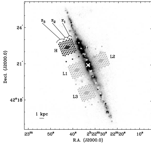
FIG. 1.—SparsePak pointings presented in this paper, overlaid on the H\alpha image of Rand et al. (1990). The spectrograph was set up in echelle mode for pointing H (black circles) and in a lower spectral resolution mode for pointings L1, L2, and L3 (gray circles). “Sky” fibers lying along the major axis are colored white for clarity. The rotational center of NGC 891 is marked with a white cross. The spatial scale (assuming D = 9.5 Mpc) is shown in the lower left. Ranges of fibers used to construct PV diagrams (see text) are marked z_1 ( 25'' < z < 45'' ), z_2 ( 45'' < z < 65'' ), and z_3 ( 65'' < z < 105'' ). These heights correspond to 1.2 \text{ kpc} < z < 2.1 \text{ kpc} , 2.1 \text{ kpc} < z < 3.0 \text{ kpc} , and 3.0 \text{ kpc} < z < 4.8 \text{ kpc} , respectively.
