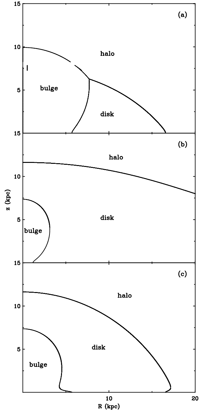
FIG. 10.—Depictions of the regions in the ballistic model within which the disk, bulge, and halo potentials contribute the most to the ( a ) radial component of the gravitational acceleration, ( b ) the vertical component of the gravitational acceleration, and ( c ) the total gravitational acceleration.
