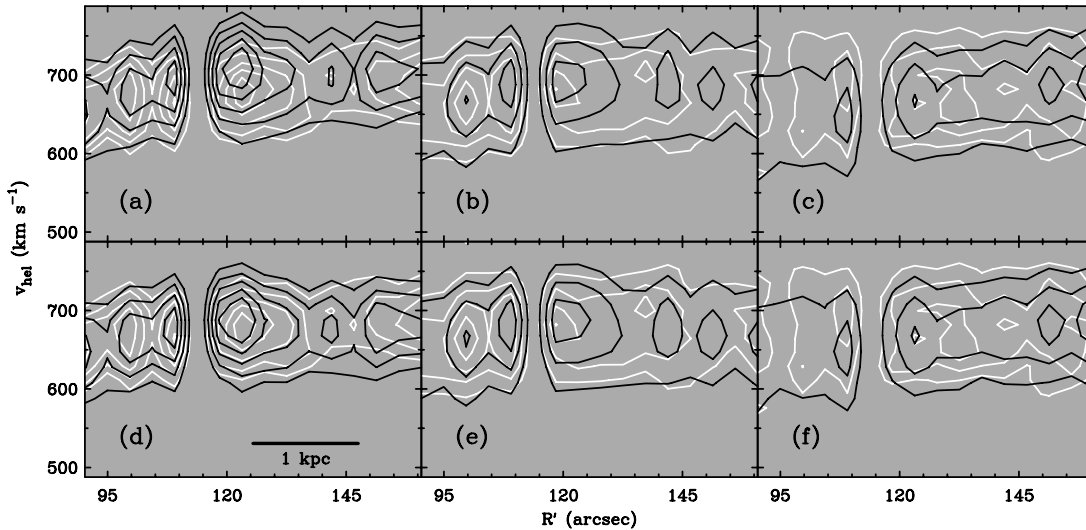
FIG. 5.— Comparison between PV diagrams constructed from pointing L3 ( white contours ) and two models: one including a gradient 15 \text{ km s}^{-1} \text{ kpc}^{-1} as described in the text ( black contours, top ) and the other including a constant rotation speed with height V_{\text{rot}}(R, z) = 175 \text{ km s}^{-1} ( black contours, bottom ). Contour levels are (a, d) 10\text{--}30 \sigma in increments of 5 \sigma for 25'' < z < 45'' , (b, e) 5\text{--}20 \sigma in increments of 5 \sigma for 45'' < z < 65'' , and (c, f) 3\text{--}9 \sigma in increments of 3 \sigma for 65'' < z < 105'' . Pointing L3 is on the receding side of the galaxy; the systemic velocity is 528 \text{ km s}^{-1} . The sky coordinate R' increases to the south. The angular size corresponding to 1 kpc is shown in the bottom left panel.
