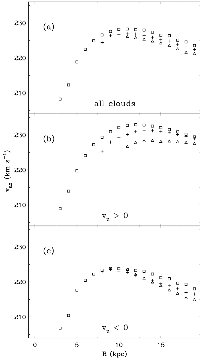
FIG. 6.—Azimuthal velocities extracted from the ballistic base model for (a) all clouds, (b) clouds moving upward (away from the disk), and (c) clouds moving downward (toward the disk). The rotation curves are averages computed within 1.2 \text{ kpc} < z < 2.1 \text{ kpc} (squares), 2.1 \text{ kpc} < z < 3.0 \text{ kpc} (plus signs), and 3.0 \text{ kpc} < z < 4.8 \text{ kpc} (triangles).
