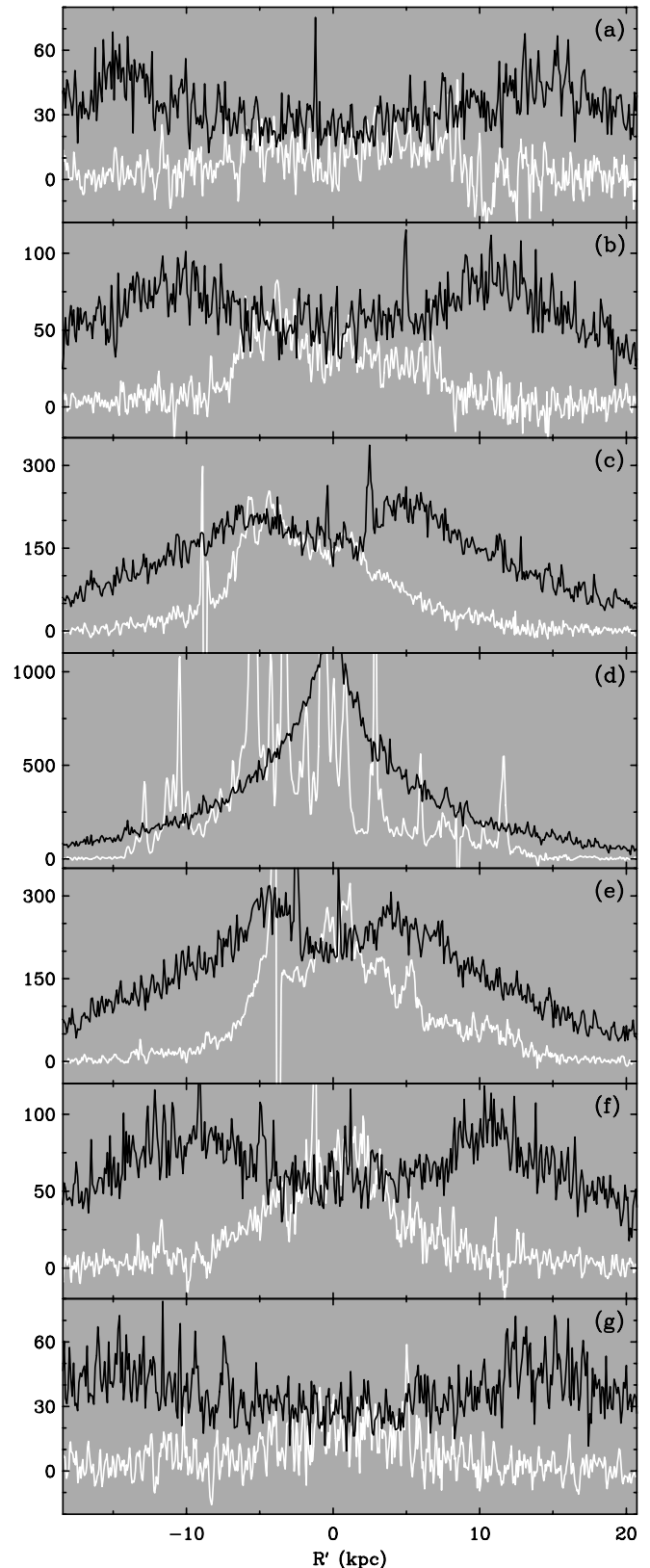
FIG. 7.—Intensity profiles along cuts through the ballistic model (black lines) and the \text{H}\alpha data (white lines). The vertical scale is in units of emission measure ( \text{pc cm}^{-6} ) for the \text{H}\alpha data and number of clouds (multiplied by a constant for presentation) for the ballistic model data. The cuts were made parallel to the major axis at heights (a) z = 3 \text{ kpc} (to the east of the disk), (b) z = 2 \text{ kpc} (east), (c) z = 1 \text{ kpc} (east), (d) z = 0 \text{ kpc} , (e) z = 1 \text{ kpc} (west), (f) z = 2 \text{ kpc} (west), and (g) z = 3 \text{ kpc} (west). The sky coordinate R' increases to the south.
