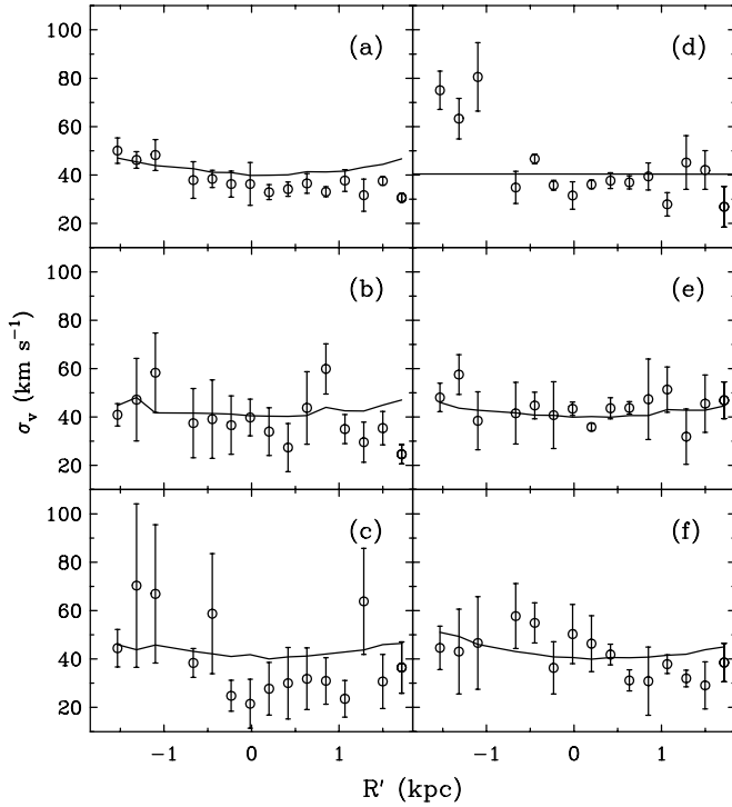
FIG. 8.— H\alpha velocity dispersions ( circles ) from pointings L1 ( a-c ) and L2 ( d-f ), and velocity dispersions measured from the best-fit model described in § 3.2 ( solid lines ), which was modified to correct for the instrumental broadening (making the dispersion in the model 40 \text{ km s}^{-1} ). Widths were calculated using PV diagrams constructed at heights ( a, d ) 1.2 \text{ kpc} < z < 2.1 \text{ kpc} , ( b, e ) 2.1 \text{ kpc} < z < 3.0 \text{ kpc} , and ( c, f ) 3.0 \text{ kpc} < z < 4.8 \text{ kpc} . Errors on the model line widths are typically about 0.5\text{--}1 \text{ km s}^{-1} . For R' > +0.9 \text{ kpc} , the H\alpha widths should be considered lower limits due to confusion with a skyline. The exceptionally high data points in ( d ) are due to confusion with another, fainter skyline and should be disregarded.
