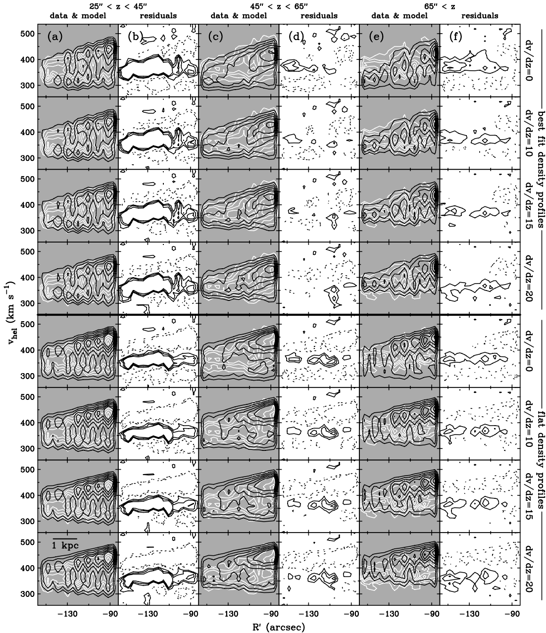
FIG. 4.— Comparison between PV diagrams constructed from the SparsePak data and from the galaxy models described in § 3.2. In the left panels ( a , c , e ) of each pair of columns, the data are shown with white contours, and the models are displayed with black contours. In the right panels ( b , d , f ), the difference between data and model is shown. The leftmost columns ( a , b ) are for heights 25'' < z < 45'' , the central columns ( c , d ) for 45'' < z < 65'' , and the rightmost columns ( e , f ) for 65'' < z < 105'' . The top four rows include models constructed using the best-fit radial density profiles shown in Fig. 3; the bottom four rows include models constructed using flat radial density profiles. The azimuthal velocity gradient used in the models in each row is listed on the right edge. From left to right, the contour levels in each column are ( a ) 10\text{--}40\sigma in increments of 5\sigma ; ( b ) 3, 5, and 7\sigma (positive for solid contours, negative for dashed contours); ( c ) 5\text{--}20\sigma in increments of 3\sigma ; ( d ) same as in ( b ); ( e ) 3\text{--}12\sigma in increments of 1.5\sigma ; and ( f ) 2, 4, and 6\sigma (positive for solid contours, negative for dashed contours). The systemic velocity is 528\text{ km s}^{-1} . The sky coordinate |R'| increases to the north. The angular size corresponding to 1\text{ kpc} is shown in the bottom left panel.
