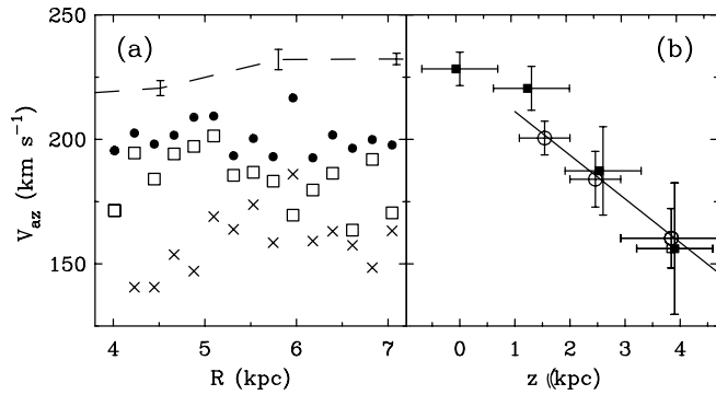
FIG. 2.—Results of applying the envelope tracing method to PV diagrams constructed from the spectra obtained in pointing H (northeast quadrant). (a) Rotational velocities for 1.2 \text{ kpc} < z < 2.1 \text{ kpc} (circles), 2.1 \text{ kpc} < z < 3.0 \text{ kpc} (squares), and 3.0 \text{ kpc} < z < 4.8 \text{ kpc} (crosses). A major-axis rotation curve determined from H I observations is included for reference (dashed line). (b) The average rotational velocity at each height is shown for the DIG (circles) and for the H I (for radii included in pointing H; squares). Horizontal errors for the DIG data indicate the range of z covered by the fibers used to construct the individual PV diagrams; those for the H I data reflect the angular resolution ( 30'' = 1.4 \text{ kpc} ). The best-fit solution for the DIG ( dv/dz = 17.5 \pm 5.9 \text{ km s}^{-1} \text{ kpc}^{-1} ), described in the text, is plotted for reference (solid line). The H I data were kindly provided by F. Fraternali.
