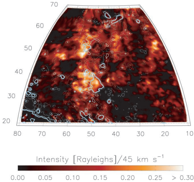
FIG. 1.—Ionized and neutral components of Complex K. Integrated H\alpha emission from v_{\text{LSR}} = -95 to -50 \text{km s}^{-1} is presented as the color image. H\text{ I} column densities (integrated over the same velocity range) of 7, 14, and 21 \times 10^{18} \text{ cm}^{-2} from Hartmann & Burton (1997) are displayed as light blue contours.
