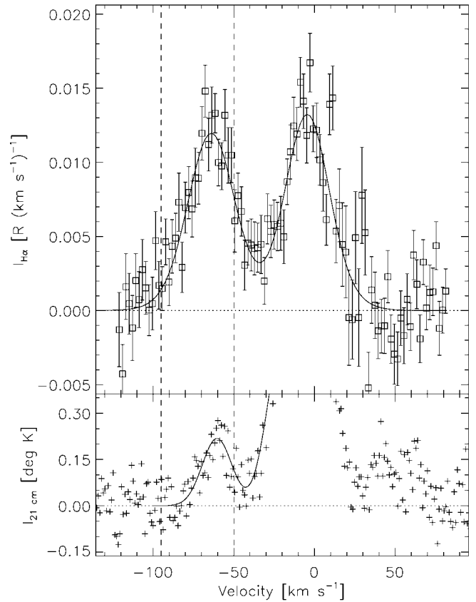
FIG. 2.— Top : WHAM H\alpha spectrum of the 1^\circ portion of the sky centered at l = 57^\circ 02 , b = +49^\circ 22 . WHAM data is plotted as squares with 1 \sigma error bars. A 3.7 R geocoronal line centered near v_{\text{LSR}} = +30 \text{ km s}^{-1} has been removed from the spectrum. A simple two-component fit to the Galactic emission is shown as the solid line (see text). Bottom : H\text{ I} 21 cm emission spectrum toward l = 57^\circ 0 , b = +49^\circ 0 from the Leiden-Dwingeloo H\text{ I} survey. The local emission peaks off the displayed scale near 8.2 K. The solid line denotes the IVC portion of a multicomponent fit (see text). In both panels, the dashed lines denote the integration range used for the image in Fig. 1.
