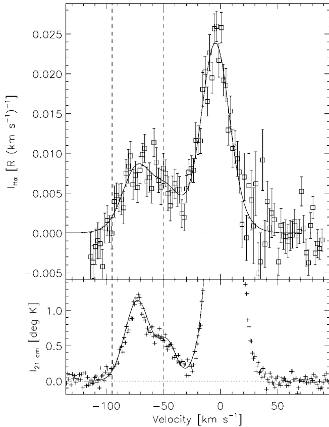
Fig. 3.—Same as Fig. 2, except toward l = 48^{\circ}03 , b = +36^{\circ}49 for H\alpha (top) and l = 48^{\circ}0 , b = +36^{\circ}5 for H\text{ I} (bottom). The local H\text{ I} emission peaks off the displayed scale near 15.8\text{ K} .
