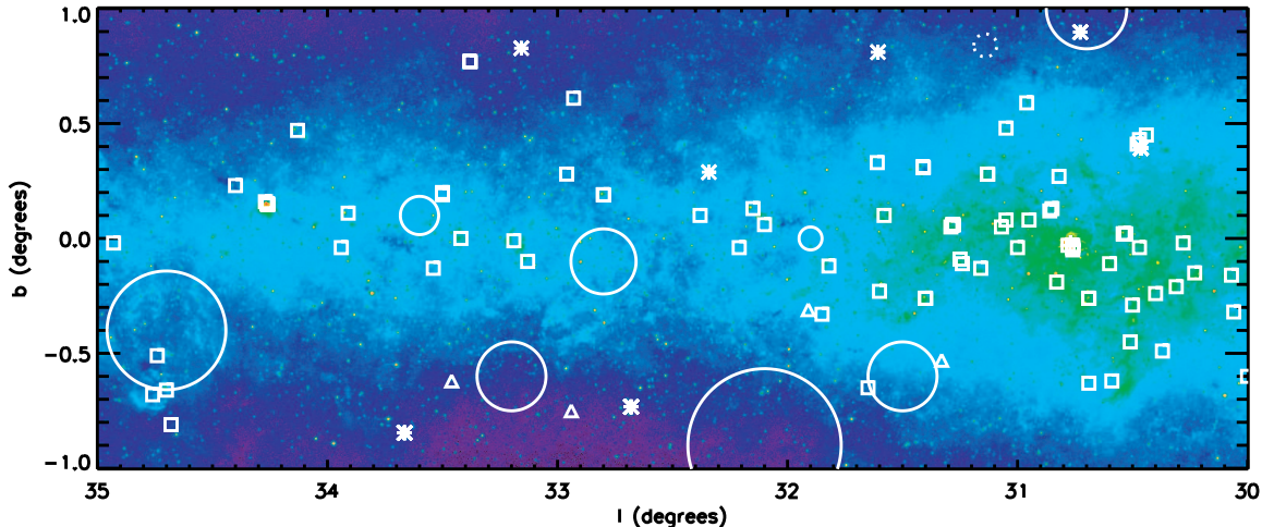
Fig. 7.— MSX 8\mu\text{m} image of a ten square degree piece of the GLIMPSE survey region, with the positions of the following classes of objects noted: OB stars (asterisks), HII regions (squares), planetary nebulae (triangles), supernova remnants (solid circles), and open clusters (dotted circles). Most of the diffuse emission in this image is due to polycyclic aromatic hydrocarbons (PAHs). The prominent star formation region at (l = 30^\circ.8, b = 0^\circ.0) is W43, which is obscured optically ( A_V \approx 30 mag). The angular resolution of MSX was 18'' as compared to the < 2'' pixel resolution expected from Spitzer /IRAC.
