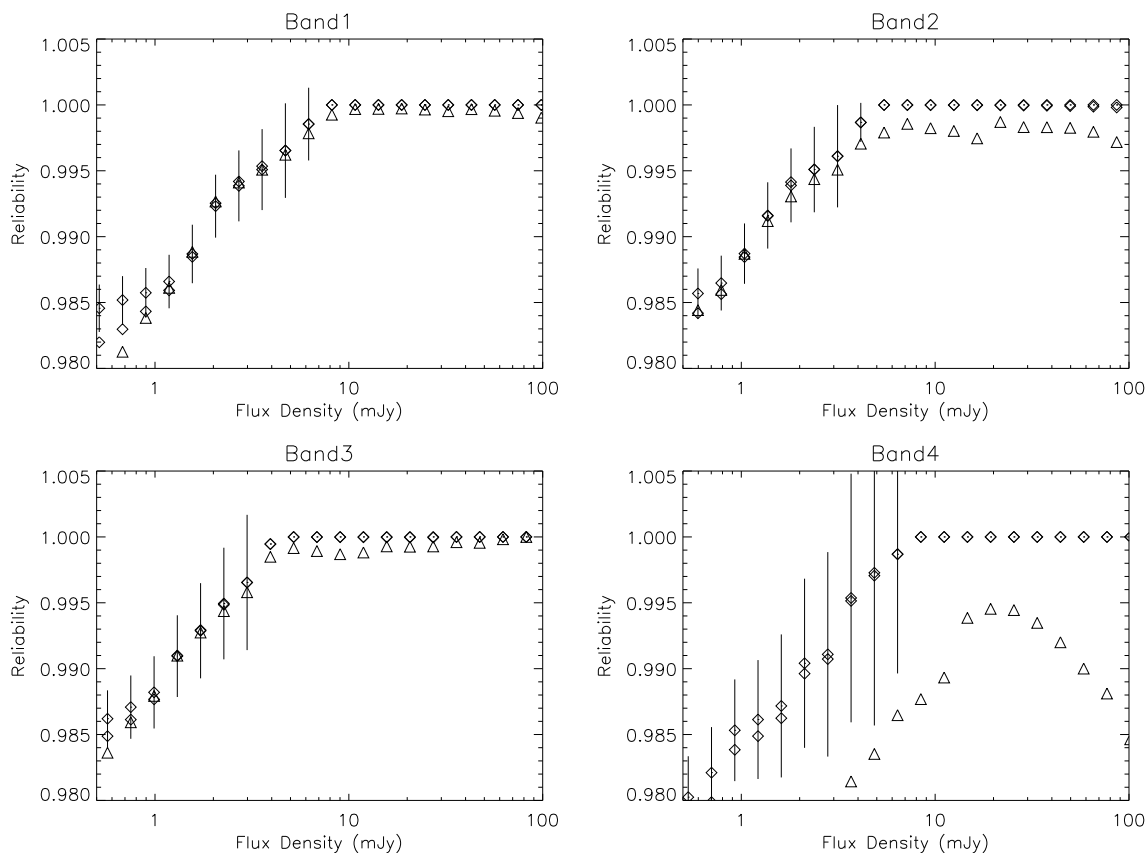
Fig. 8.— The reliability of a GLIMPSE catalog using an external truth table and three different catalog criteria. The catalog criteria are 2+2 (+), 2+1 (◇) and 2+0 (△).
