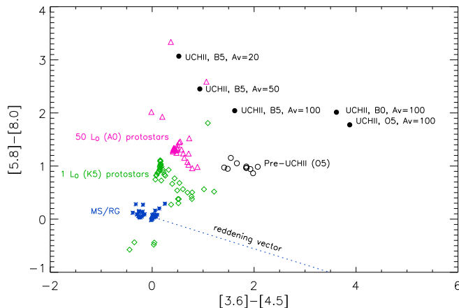
Fig. 6.— IRAC color-color diagrams of model protostars calculated by Whitney et al. (2003) with both axes in magnitudes. Filled circles are UCHII models, with various values of A(V) . The open circles are for a model of a UCHII precursor (O star embedded in an infalling envelope and accretion disk). Several viewing inclinations are plotted for this model. Open triangles show different inclination models for intermediate mass protostars (here, A0) from early protostar stage to remnant disk. Open diamonds are similar models for low mass pre-main sequence stars (K5). Only sources that are detectable to a distance of 2 kpc are plotted (i.e., the more pole-on, less reddened sources). The main sequence and giant branch are plotted as asterisks (MS), with the reddening line shown by the dotted line. Reddening is actually “blueing” in the longer wavelength bands, based on the ISM model of Li & Draine (2001) because of the strong silicate absorption features usually observed in these objects. GLIMPSE will improve our understanding of the opacity in this wavelength range.
