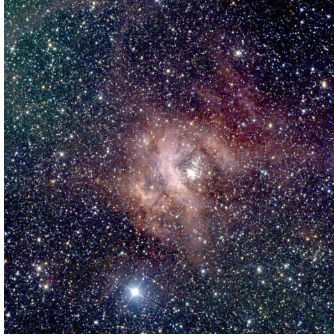
Fig. 4.— A 2MASS JHK color image of the GLIMPSE Observing Strategy Validation (OSV) area, the star formation region RCW49 ( l = 283^\circ.4 , b = -0^\circ.3 ). The image is 0.5^\circ \times 0.5^\circ . This area was observed by Spitzer in late December 2003.
