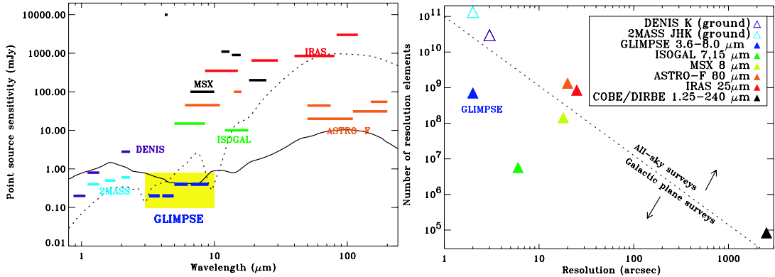
Fig. 2.— [Left panel] A comparison of the GLIMPSE sensitivity limit to the sensitivity of other ground and space-based infrared surveys. This shows the good match in sensitivity between GLIMPSE and 2MASS. The curves show model spectra of Whitney et al (2003) for a 1 L_\odot T Tauri star at a distance of 0.7 kpc (solid) and a deeply embedded 1 L_\odot protostar at a distance of 0.6 kpc (dotted). [Right panel] The number of resolution elements versus resolution for GLIMPSE and other infrared surveys. GLIMPSE will have the largest number of resolution elements of any Galactic plane-only survey, and a comparable number of resolution elements to several space-based all-sky infrared surveys.
