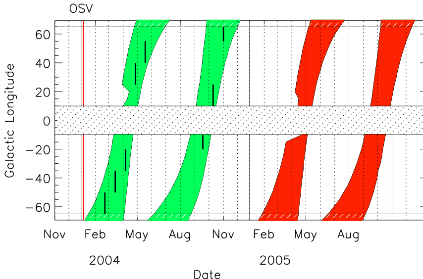
Fig. 5.— Visibility of the Galactic plane to Spitzer as a function of date and Galactic longitude. This can be used to judge when a particular part of the GLIMPSE region is likely to be observed. The planned GLIMPSE campaigns are noted with vertical bars.
